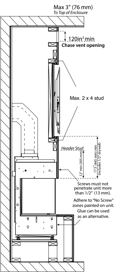
Flush wall TV recess using 1/2" (13 mm) drywall
