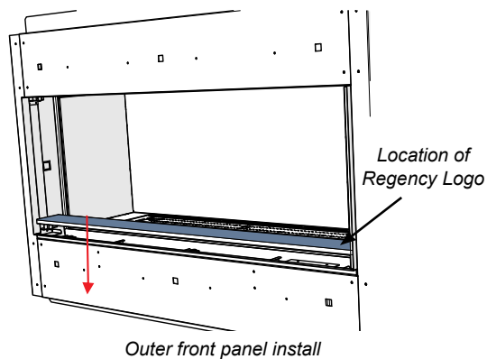
Outer front panel install
