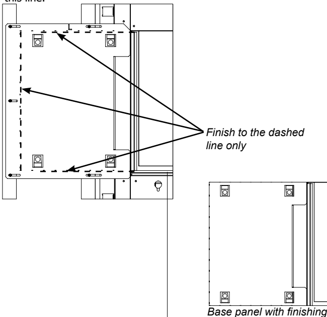
Finish wall
