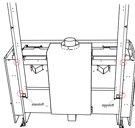
Screw Locations
