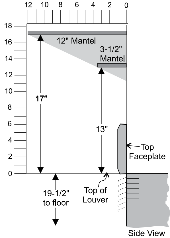
Clearances for Standard Faceplate / Low Profile Faceplate without Safety Screen
