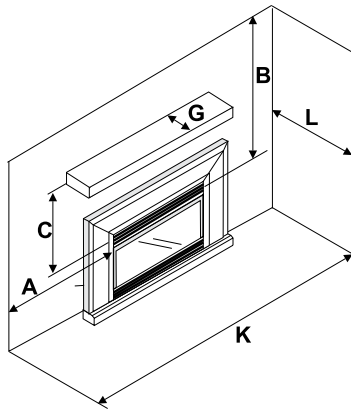
Clearances for Low Profile Faceplate with Safety Screen
