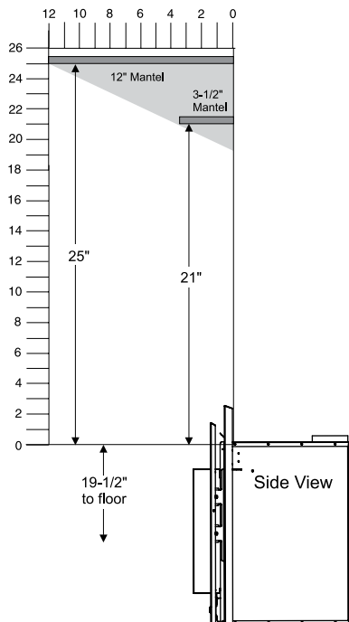
Clearances for Low Profile Faceplate with Safety Screen
