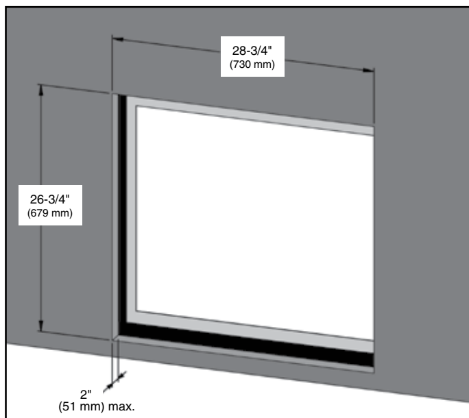
Diagram 2: Finishing Dimensions
