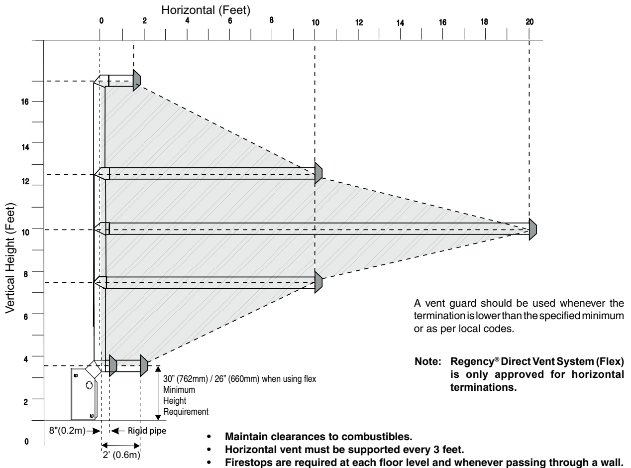
Minimum Simpson Dura-Vent Center-Line
