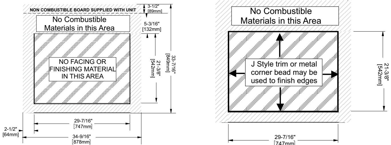
Minimum Clearances for Finishing Materials
