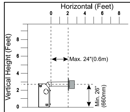
Minimum Flex Kit Center-Line
