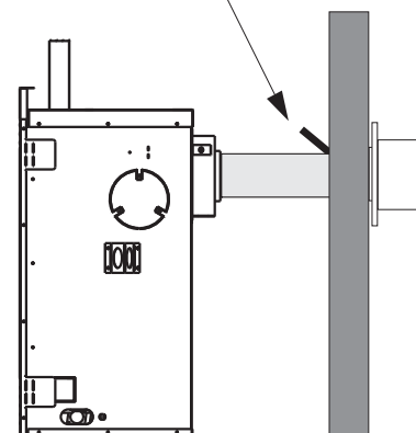
Rear Venting Deflector
