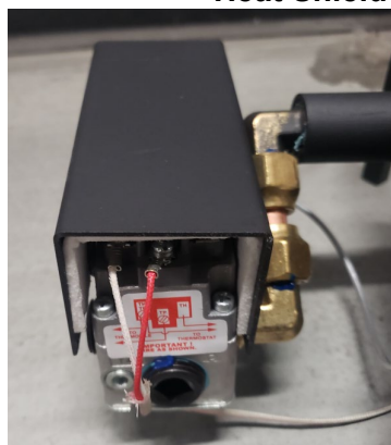
Robertshaw Millivolt Gas Valve
