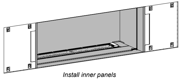
Install inner panels
