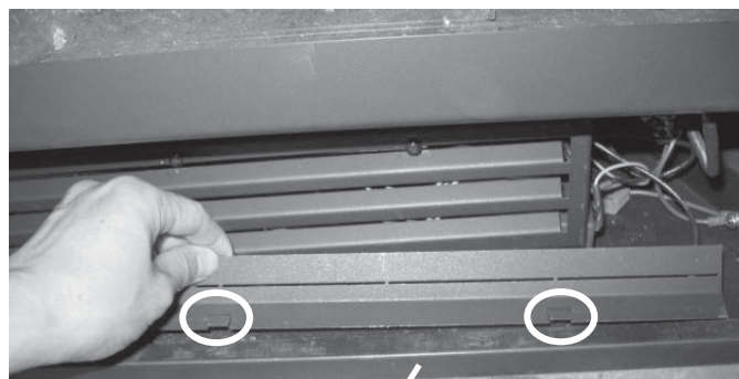
Firebox Flange
