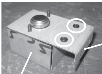
Thermdisc Cover
