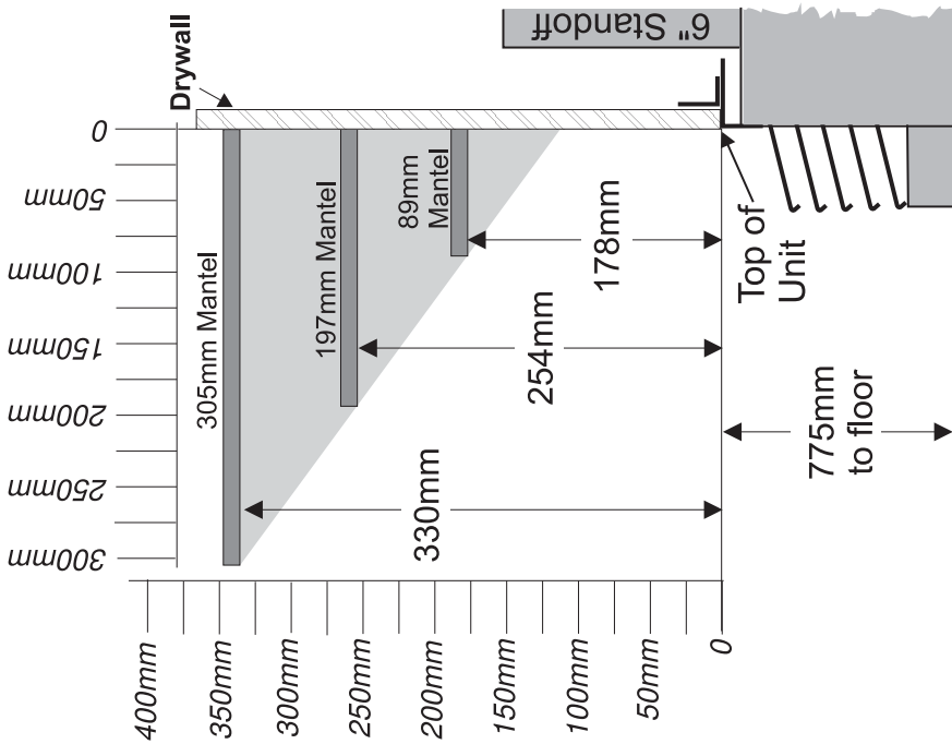
Mantel Clearances with Bay Option
