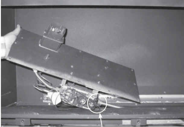
Gas Line
