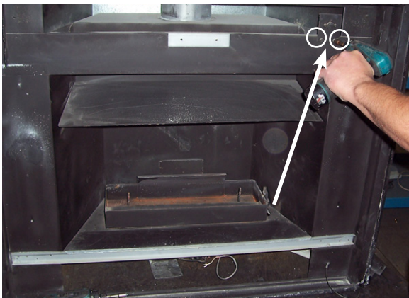
Remove 2 screws - remove Thermodisc Bracket
