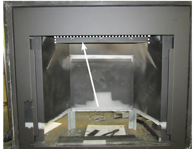
Cut out back cross bar
