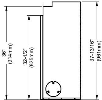
Framed opening - Side View
