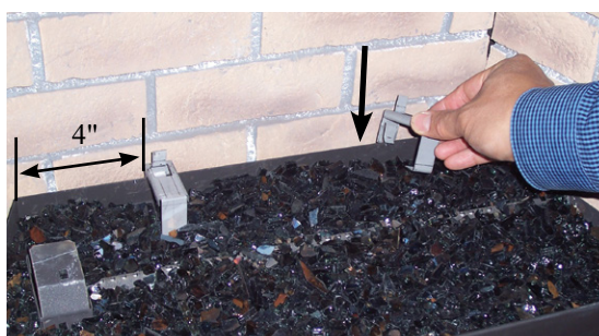
Brackets installed 4" from outside edge of burner tray
