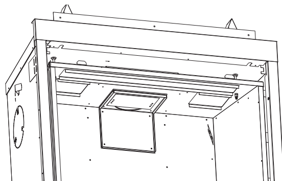
Schéma 2 Vent restrictor installed on top exhaust assembly
