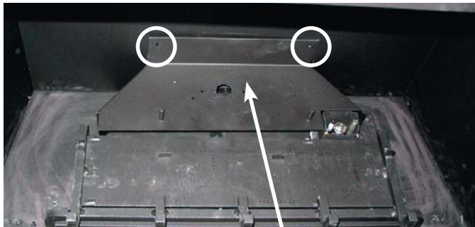
support de bûche
