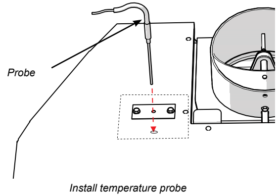
Install temperature probe
