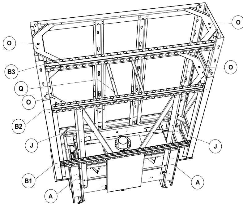
Back view Part ID - extended shown
