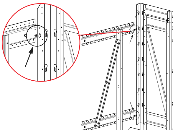
Install Pre Assembled Sidewall
