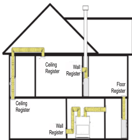
Diagram 1: Guide for possible air duct runs and locations. Keep duct length and number of bends to a minimum. Maximum duct length is 9.0m. The Fan Kit 946-591 does not contain any flueing a separate Flex Kit is required 946-596. This Flex Kit contains one length of 4.5 metres of flex flueing. If 9.0 metres of flex ducting is required you will need to purchase an additional Flex Kit.
