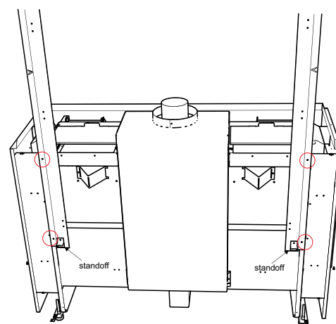
Screw Locations
