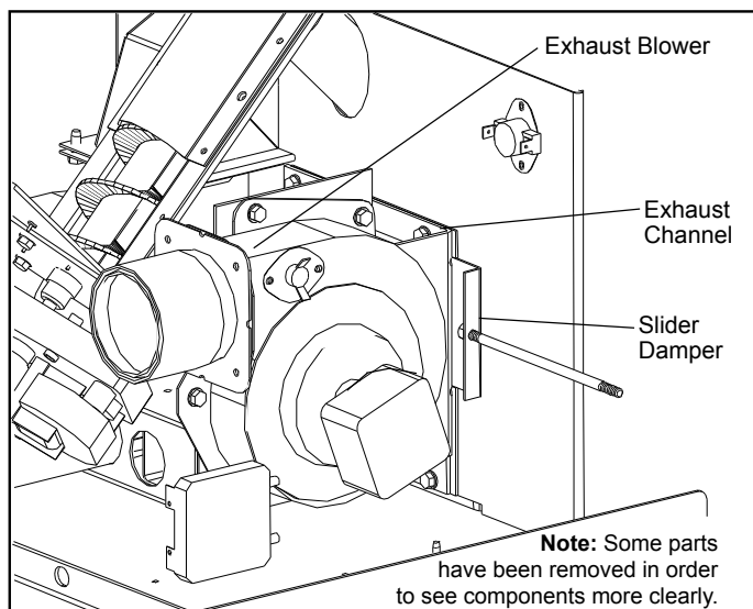
Figure 39: Slider / Damper
