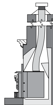
Recommended chimney height from top of flue collar: Minimum 15 feet (4.6 meters)
