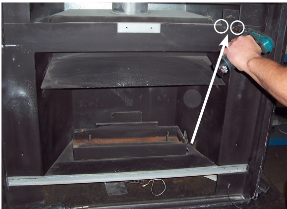
Remove 2 screws - remove Thermodisc Bracket
