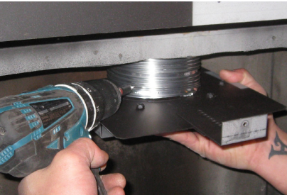
Secure vent slide plate to flex pipe with 4 screws
