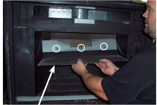
Remove 3 bolts and nuts to remove heat deflector.
