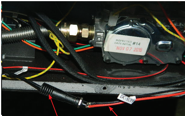
AC adaptor DC supply wire from wiring harness
