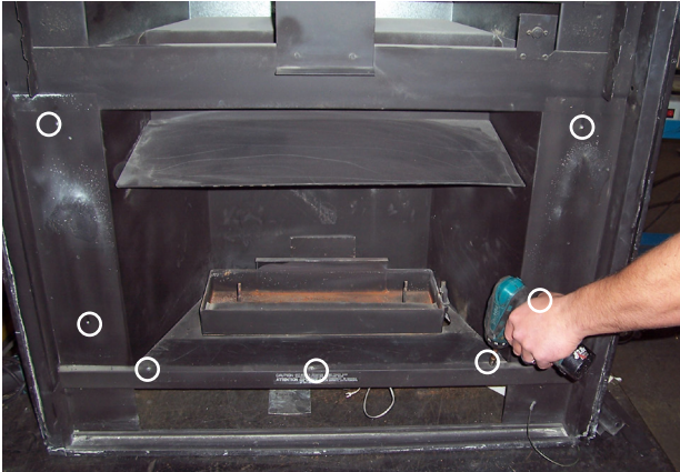
Remove 7 screws - remove Mesh Door Frame (if installed).
