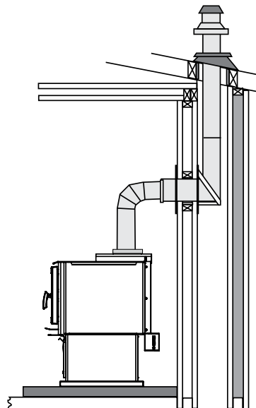
Installation horizontale
