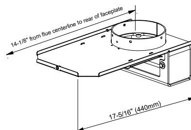
6" (152mm) Diameter OFFSET FLUE ADAPTOR (172-946)
