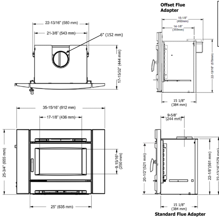
6" (152mm) Diameter STANDARD FLUE ADAPTOR (172-942)
