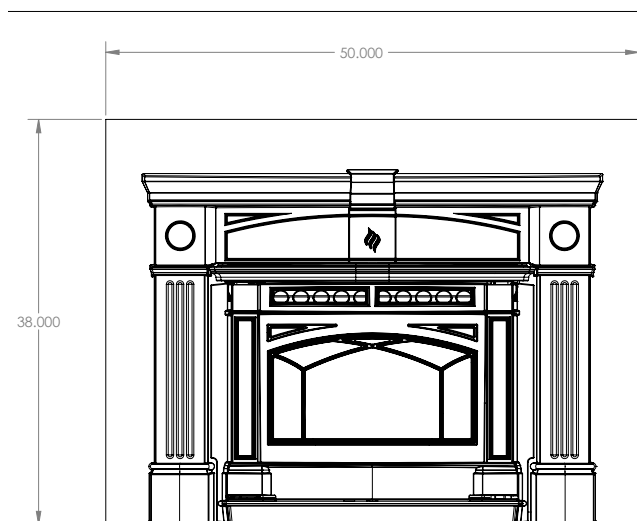
Filler Panels Dimensions
